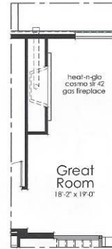
OPTIONAL COSMO GAS FIREPLACE LOCATION AT GREAT ROOM
